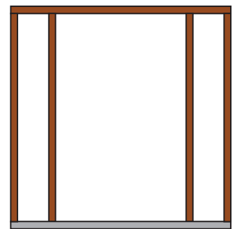
Double External Frame Plus 2 /400 Sidelights Door Opening Size: 2045 x 1630mm O/A Frame Size: 2143h x 2520mm w
