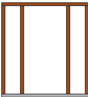
Single External Frame Plus 2 /400 Sidelight Door Opening Size: 2045 x 820mm O/A Frame Size: 2143h x 1710mm w
