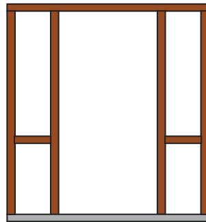
Single External Frame Plus 2 /400 Sidelight & Chair Rail Door Opening Size: 2045 x 820mm O/A Frame Size: 2143h x up to 1810mm w
