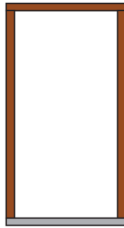
Single External Frame Door Opening Size: 2045 x 820mm O/A Frame Size: 2143h x 880mm w
