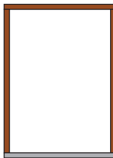
Double External Frame Door Opening Size: 2045 x 1630mm O/A Frame Size: 2143h x 1690mm w
