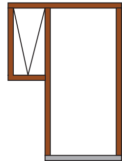
Single Winglight External Frame Unglazed (ex- cluding winder) Door Opening Size: 2045 x 820mm O/A Frame Size: 2143h x up to 1570mm w
