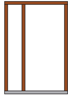
Single External Frame Plus 1 /400 Sidelight Door Opening Size: 2045 x 820mm O/A Frame Size: 2143h x 1295mm w
