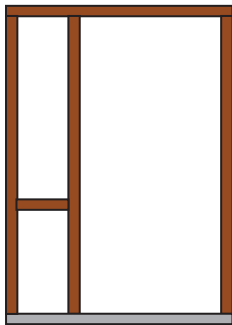
Single External Frame Plus 1 /400 Sidelight & Chair Rail Door Opening Size: 2045 x 820mm O/A Frame Size: 2143h x up to 1330mm w
