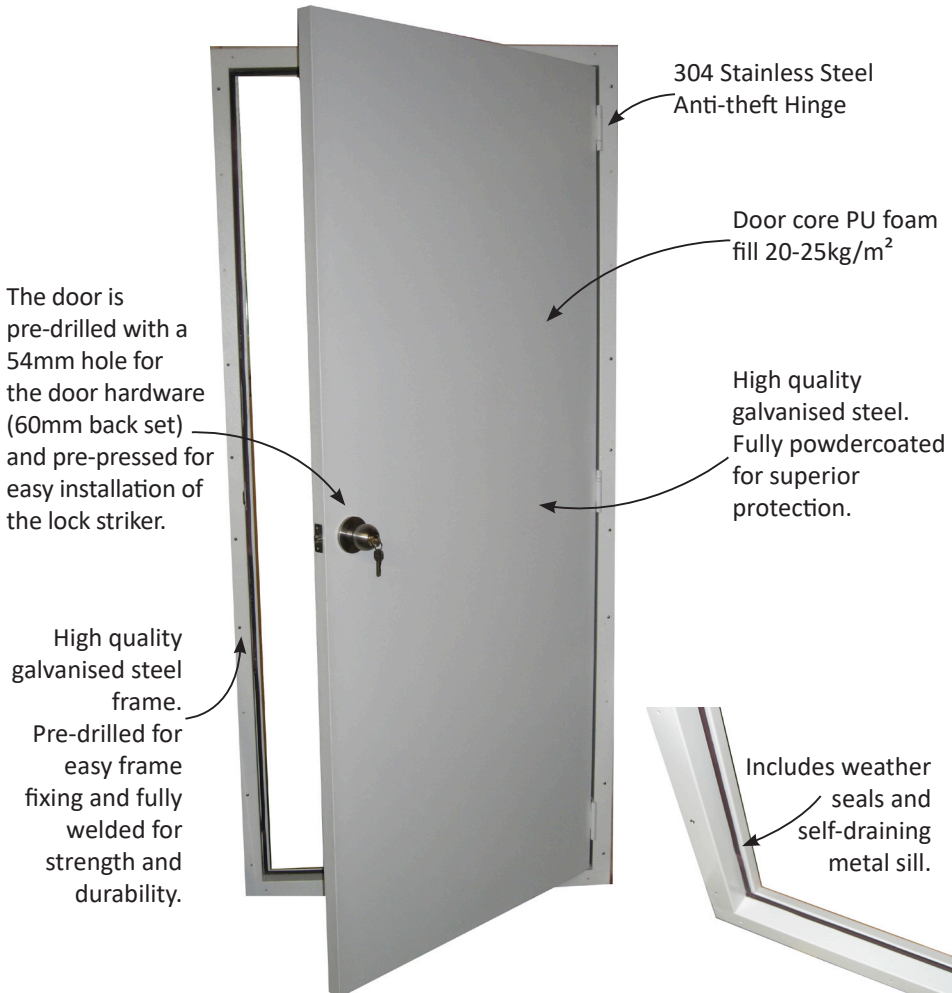
A01 ENDURO DOOR (As shown)
