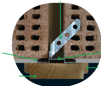
aluminium subframe + temporary pine braces + clip on aluminium brick ties
