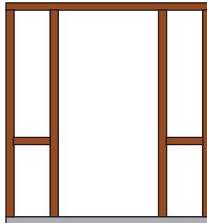
Single External Frame Plus 2/400 Sidelight & Chair Rail Door Opening Size: 2045 x 820mm O/A Frame Size: 2143h x upto 1810mm w
