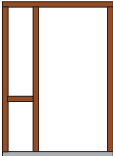
Single External Frame Plus 1/400 Sidelight & Chair Rail Door Opening Size: 2045 x 820mm O/A Frame Size: 2143h x upto 1330mm w
