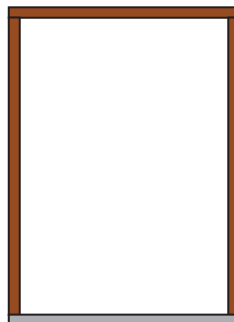
Double External Frame Door Opening Size: 2045 x 1630mm O/A Frame Size: 2143h x 1690mm w
